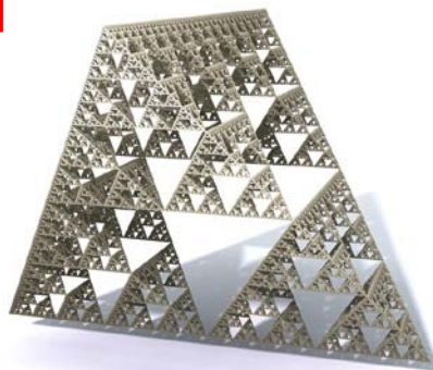
fractale 3D de Sierpinski IS
